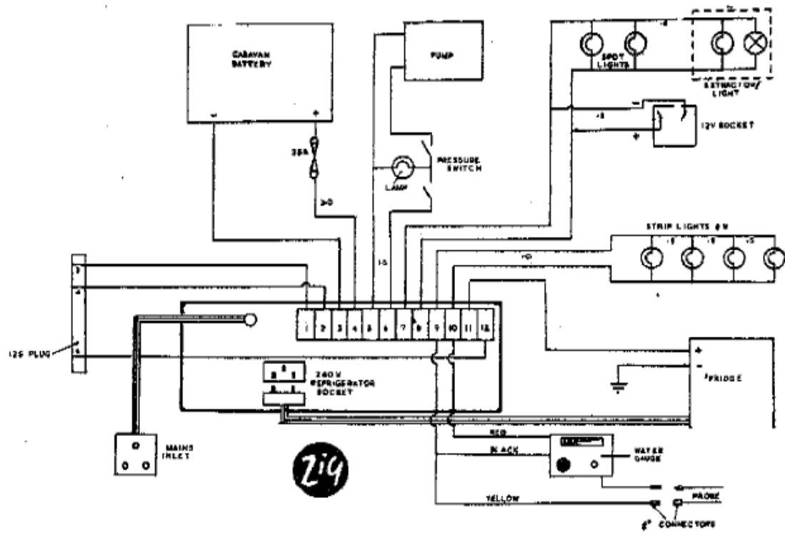
Figure 3. Suggested wiring diagram for C.F.9
