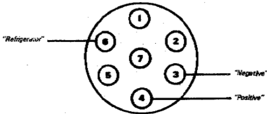
Figure 4. 12S plug
