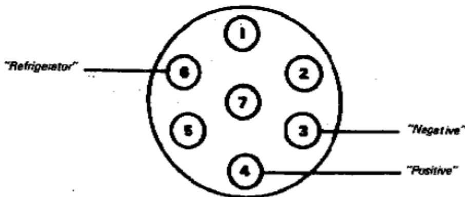
Figure 2. 12S plug
